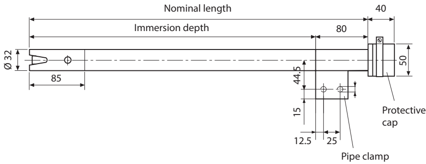
Pipe clamp
