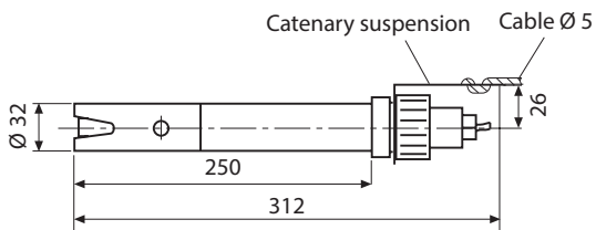
Catenary suspension
