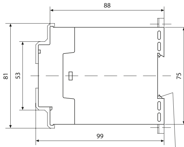
Snap-on mounting on 35-mm DIN rail to EN 60715
