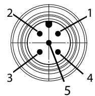
M12 connector
